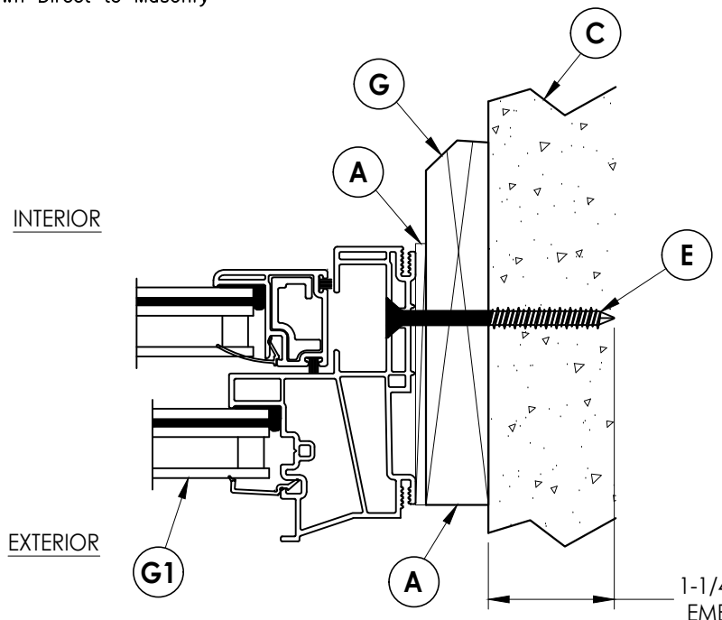
2/2 HORIZONTAL CROSS SECTION Shown w/ 1X Stud Construction
