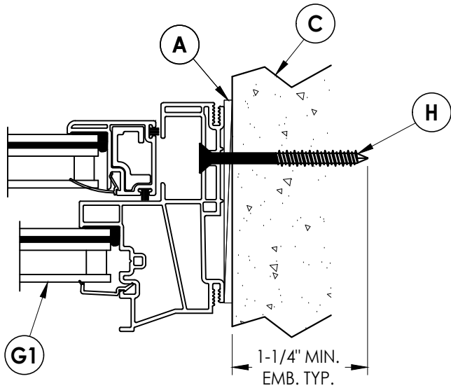
4/2 HORIZONTAL CROSS SECTION Shown Direct to Masonry
